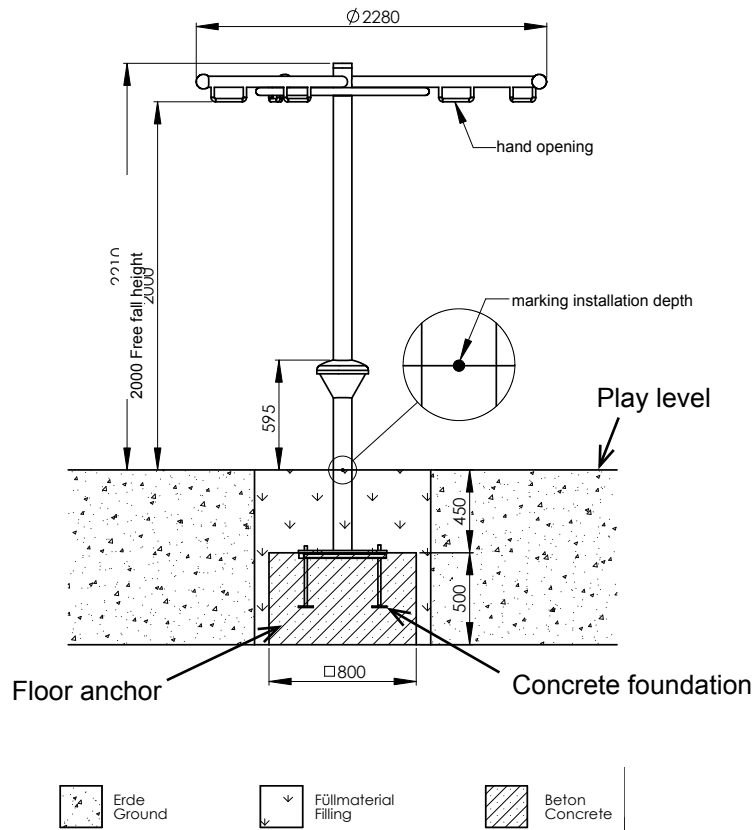
Diagram 2: Side view with dimension details „ventus“
