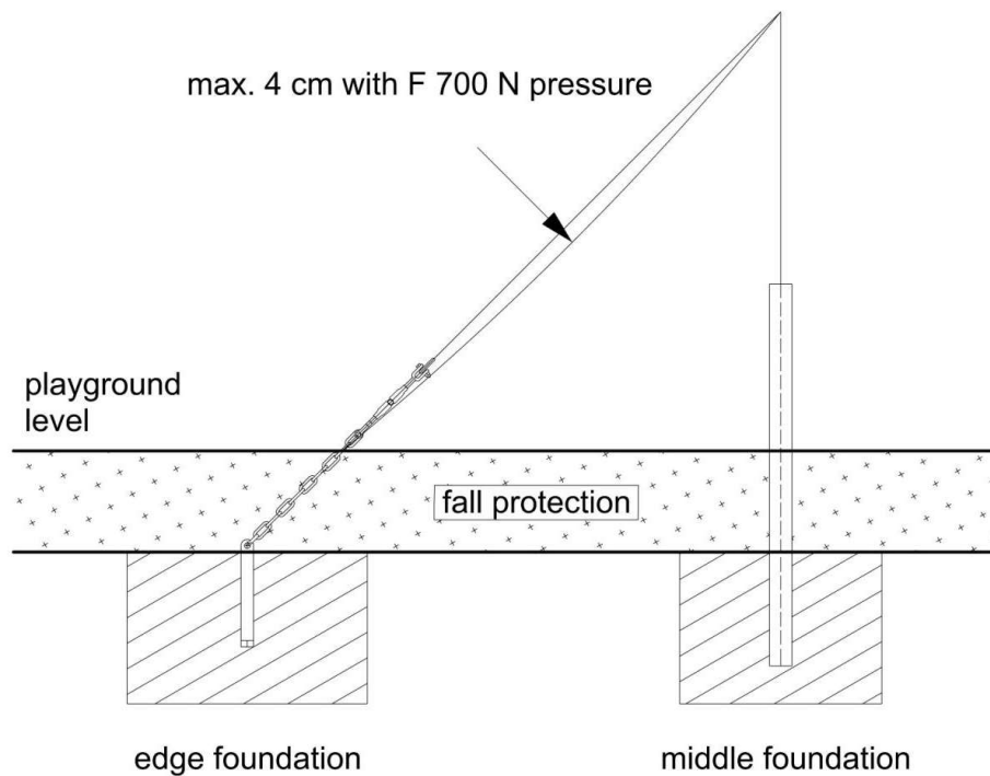
Drawing 6: Pressure-load test
