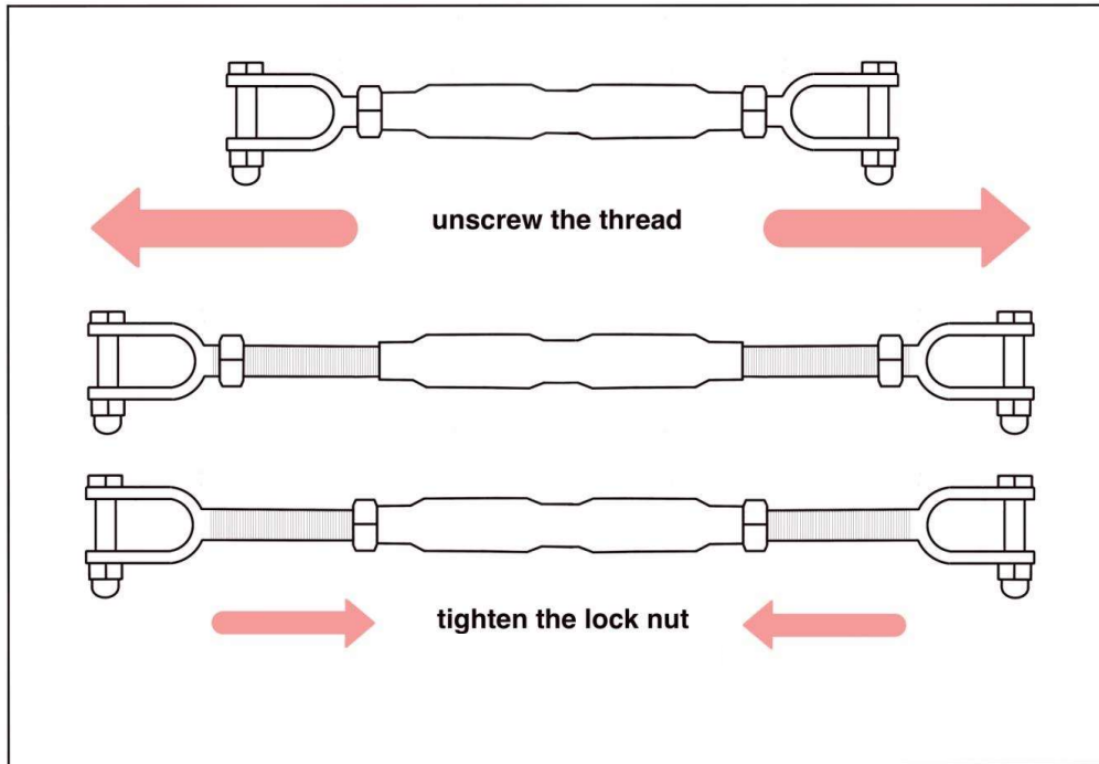
Drawing 5: Functional principle of a turnbuckle
