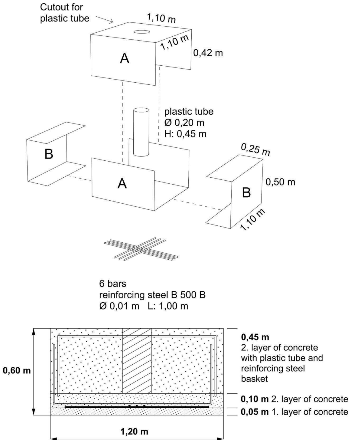
Drawing 1: Production and position of the reinforcing steel bars and the Reinforcement basket for the middle foundation
