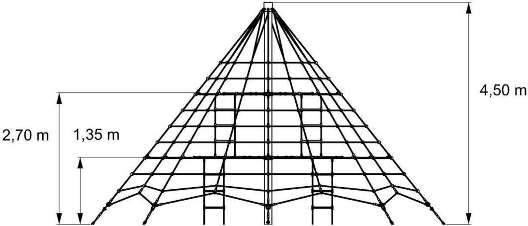
Drawing 7: Front view with net level
